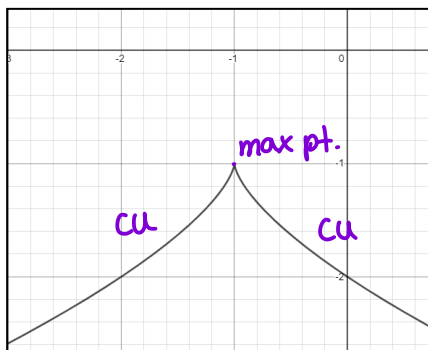
cusp (maximum)
