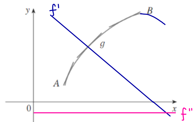
Concave Down
