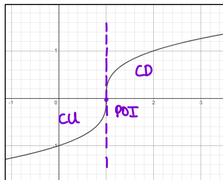
vertical tangent
