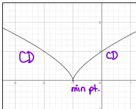
cusp (minimum)
